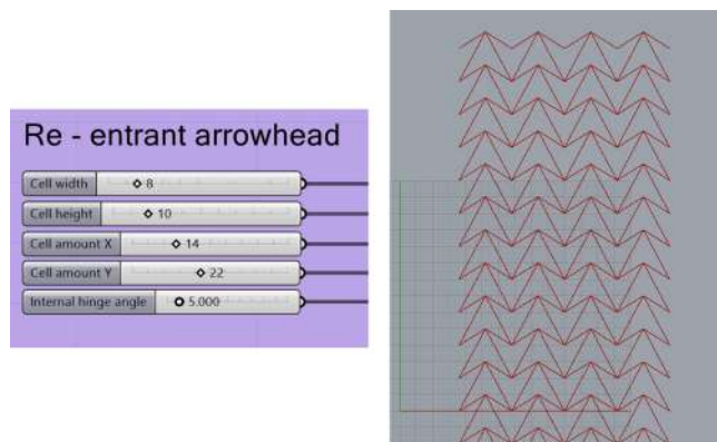
Figure 2: Preview of the auxetic re-entrant arrowhead elastomer toolpath created with a parametric code in Grasshopper for Rhino 3D, including the auxetic cell parameter sliders.
