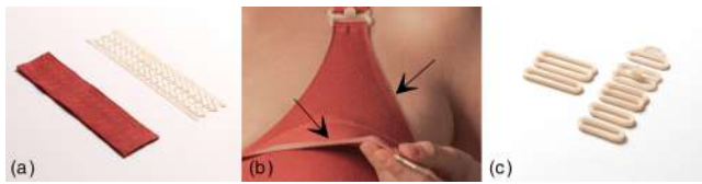
Figure 4: (a) Printed auxetic elastic band with and without the cotton knit fabric encapsulation, (b) Laser cut edge for eliminating hems and reducing bulk for the nursing mechanism, (c) 3D printed slider adjusters and nursing clips.
